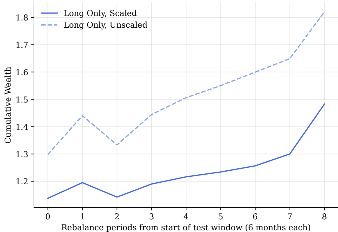
FT-Transformer, Long Only
