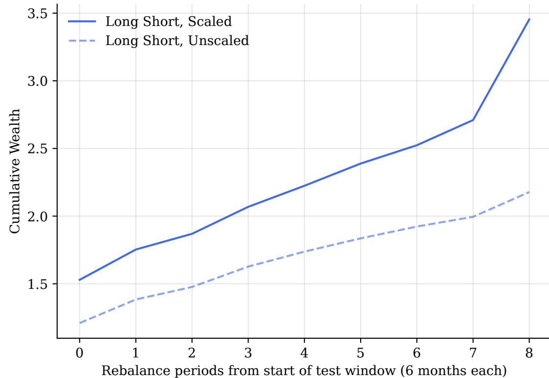
FT-Transformer, Long Short
