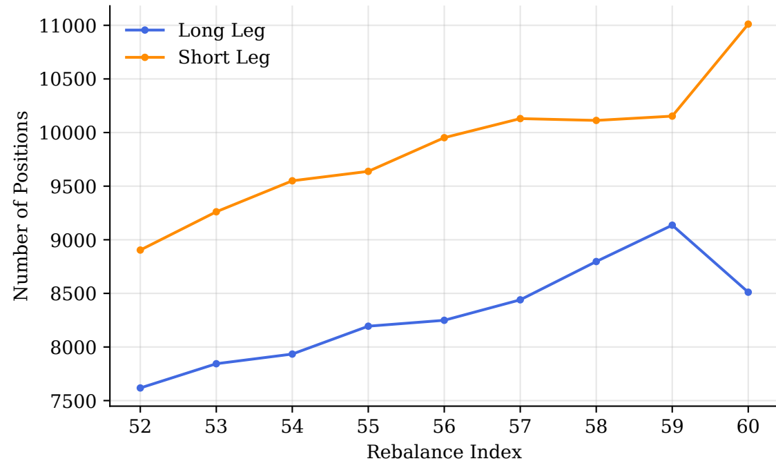
FT-Transformer, Long Short Leg Sizes Over Time
