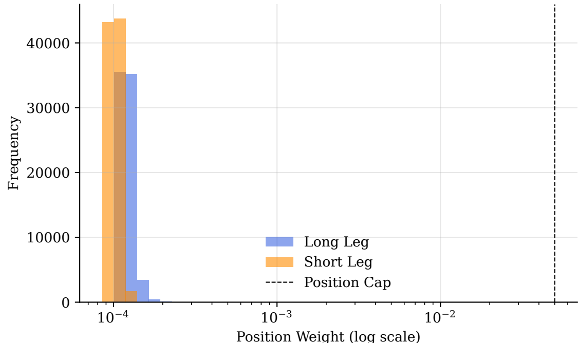
FT-Transformer, Position Weight Distribution
