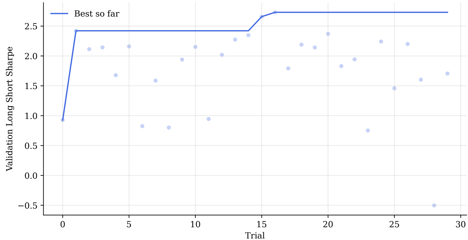
FT-Transformer Hyperparameter Search
