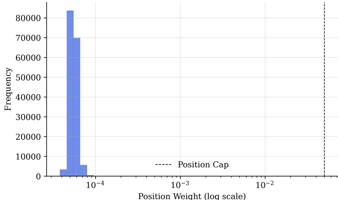
FT-Transformer, Long Only Position Weight Distribution
