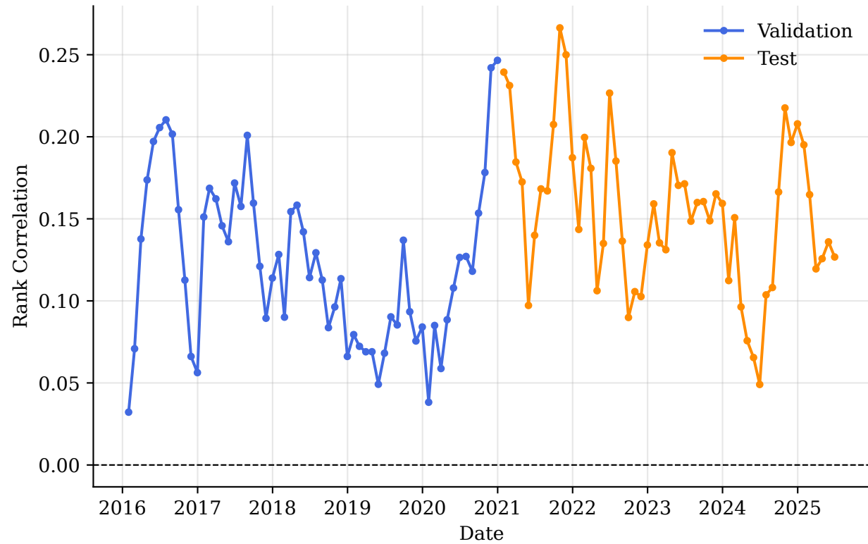
FT-Transformer, Monthly Rank Correlation, Validation Versus Test
