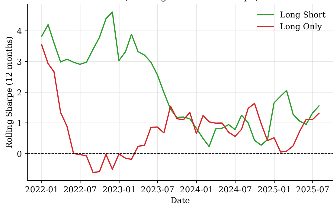
MLP Portfolios, Rolling 12-Month Sharpe, Unscaled
