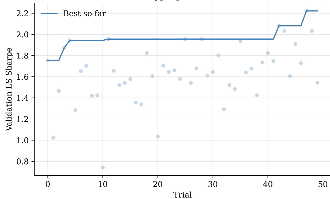
XGBoost Hyperparameter Search
