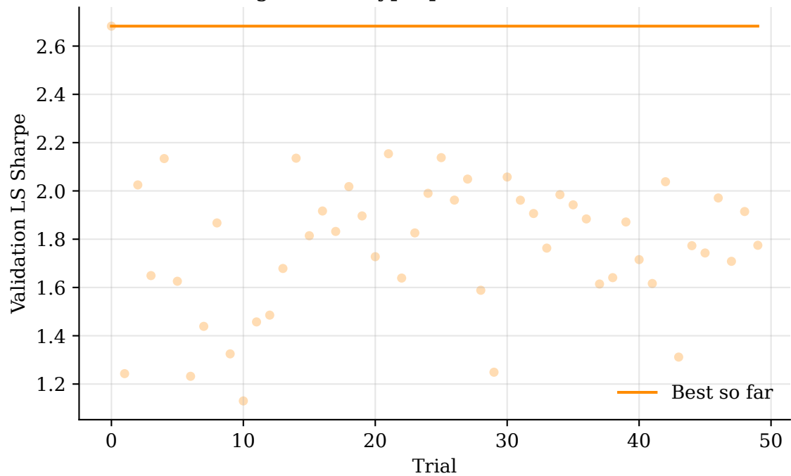
LightGBM Hyperparameter Search
