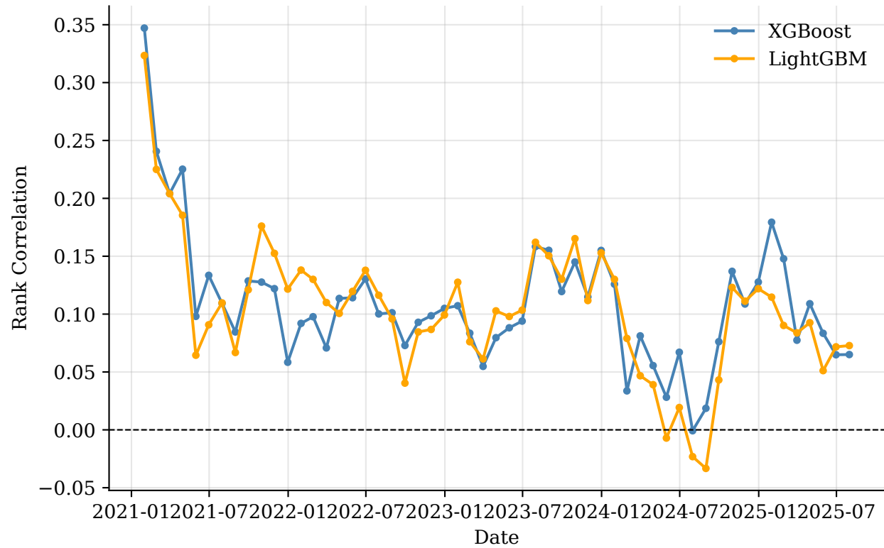
Tree Models, Monthly Rank Correlation, Test Set
