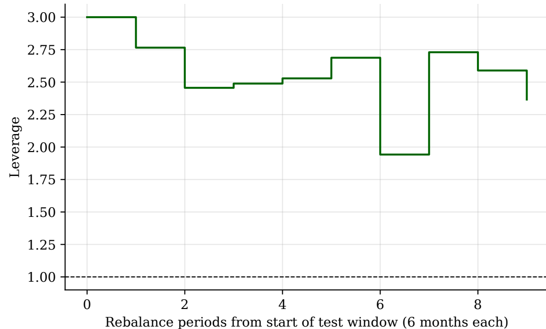
Long Short, Volatility Overlay Leverage
