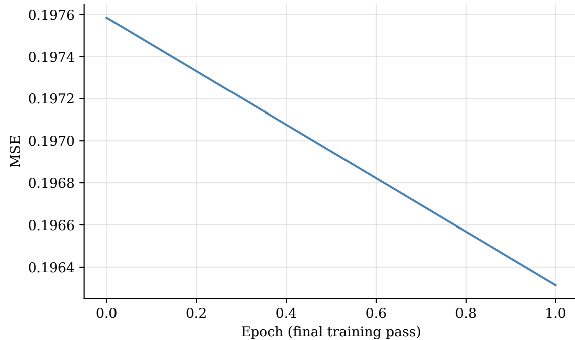
Training Loss
