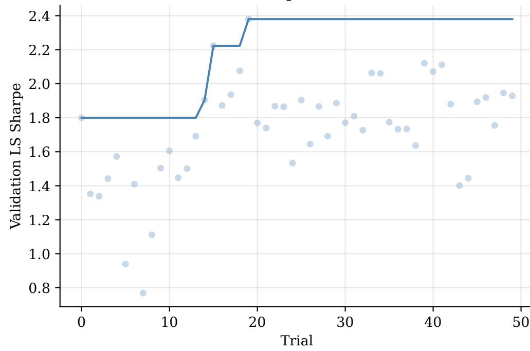
XGBoost Optuna Search
