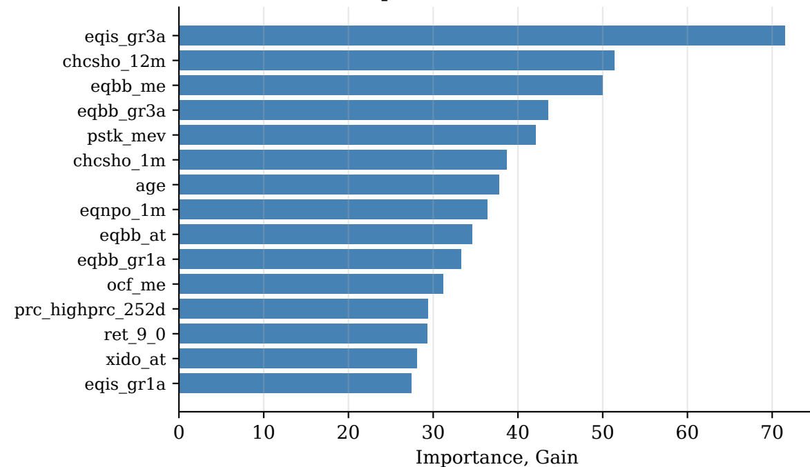
Top 15 XGBoost Features
