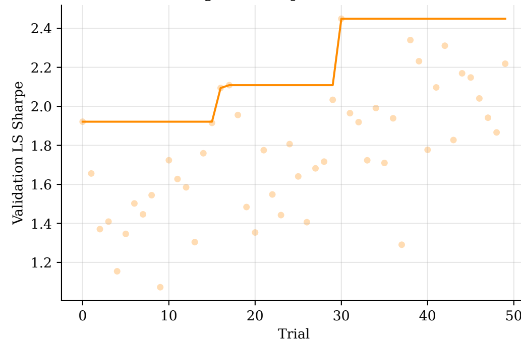
LightGBM Optuna Search
