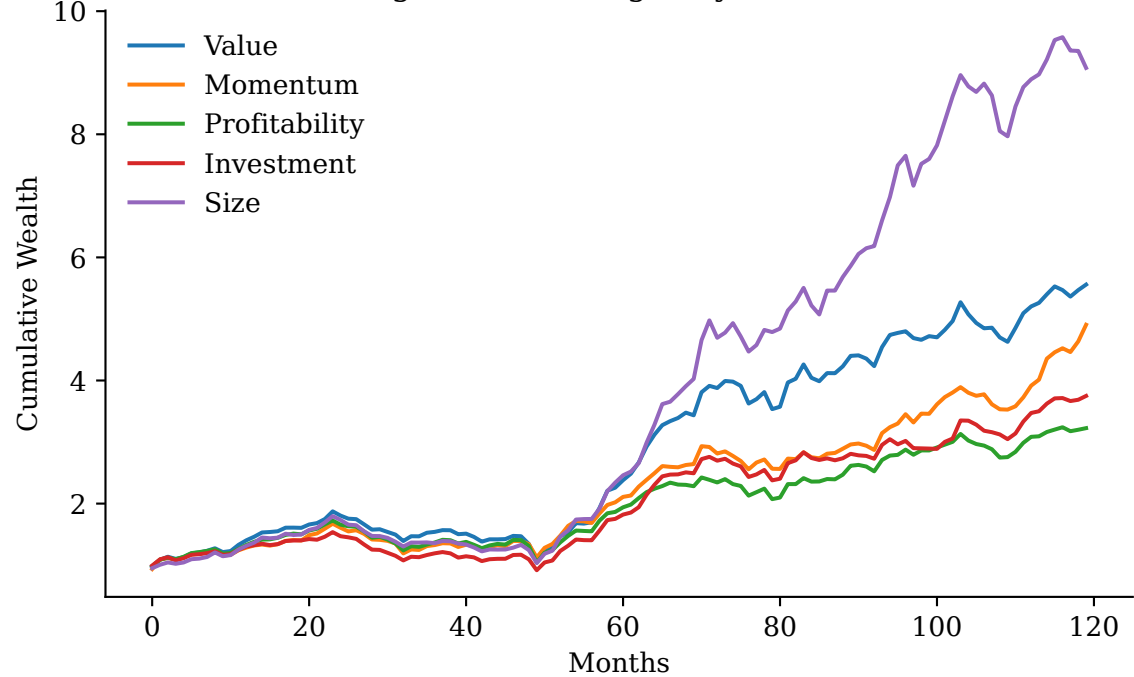
Single Factor Long Only, Unscaled
