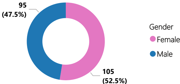
Gender-wise Admissions
