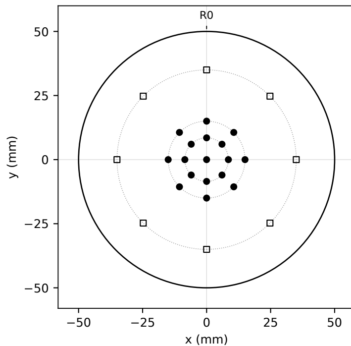
(b) S02: Ø 100 mm, thickness 100 mm End face A
