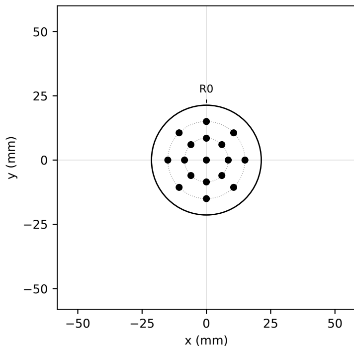
(a) S01: Ø 42.7 mm, thickness 30 mm End face A
