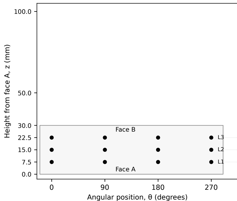
(c) S01: lateral surface
