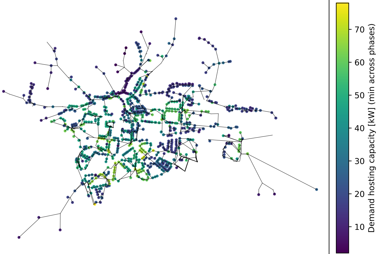
Demand nodal hosting capacity at critical hour (t=12)
