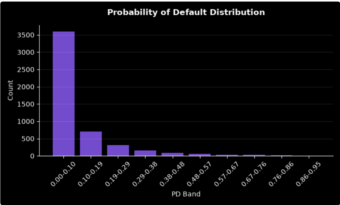
CHART_PD_DISTRIBUTION
