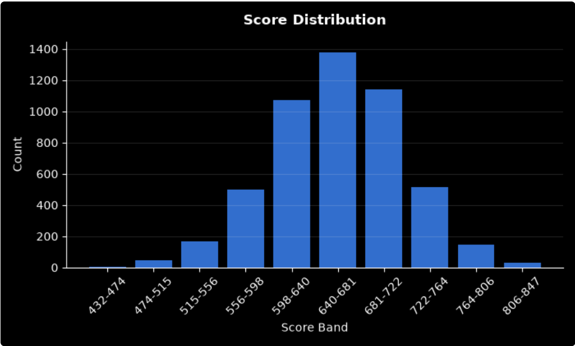
CHART_SCORE_DISTRIBUTION
