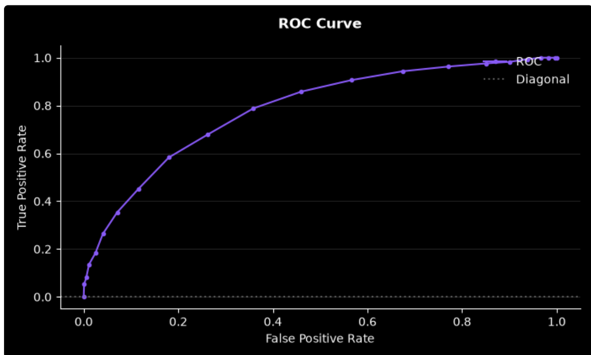
CHART_ROC_CURVE
