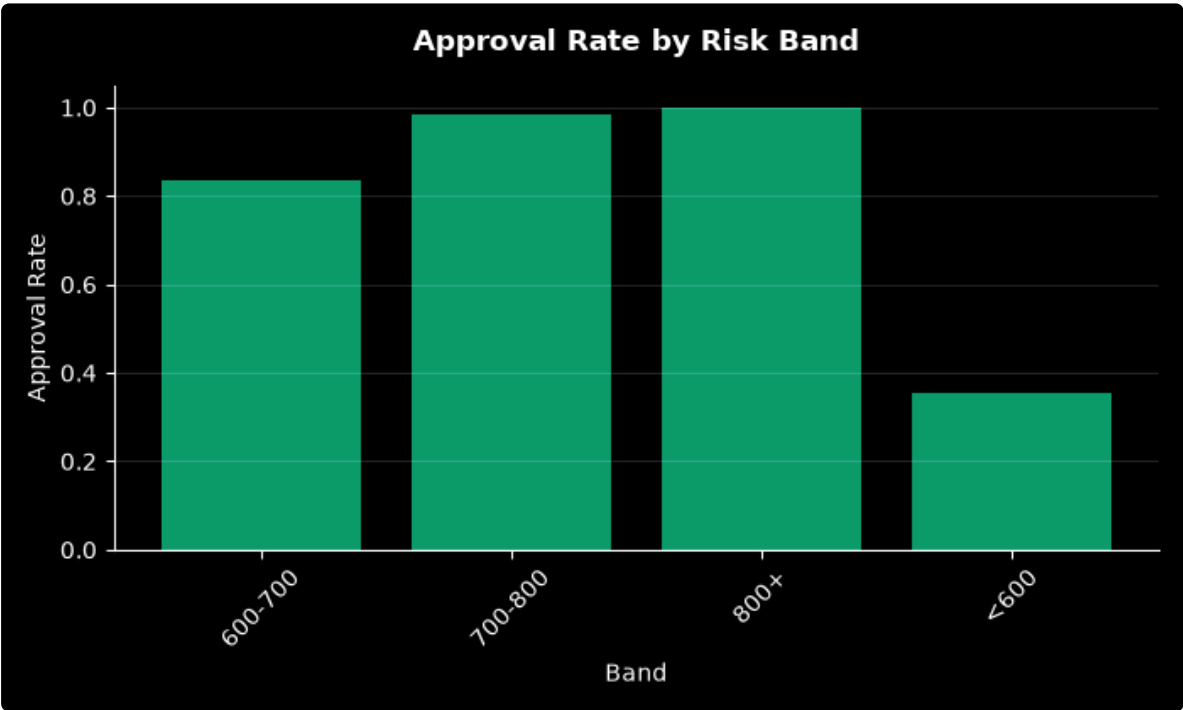
CHART_APPROVAL_BY_RISK_BAND
