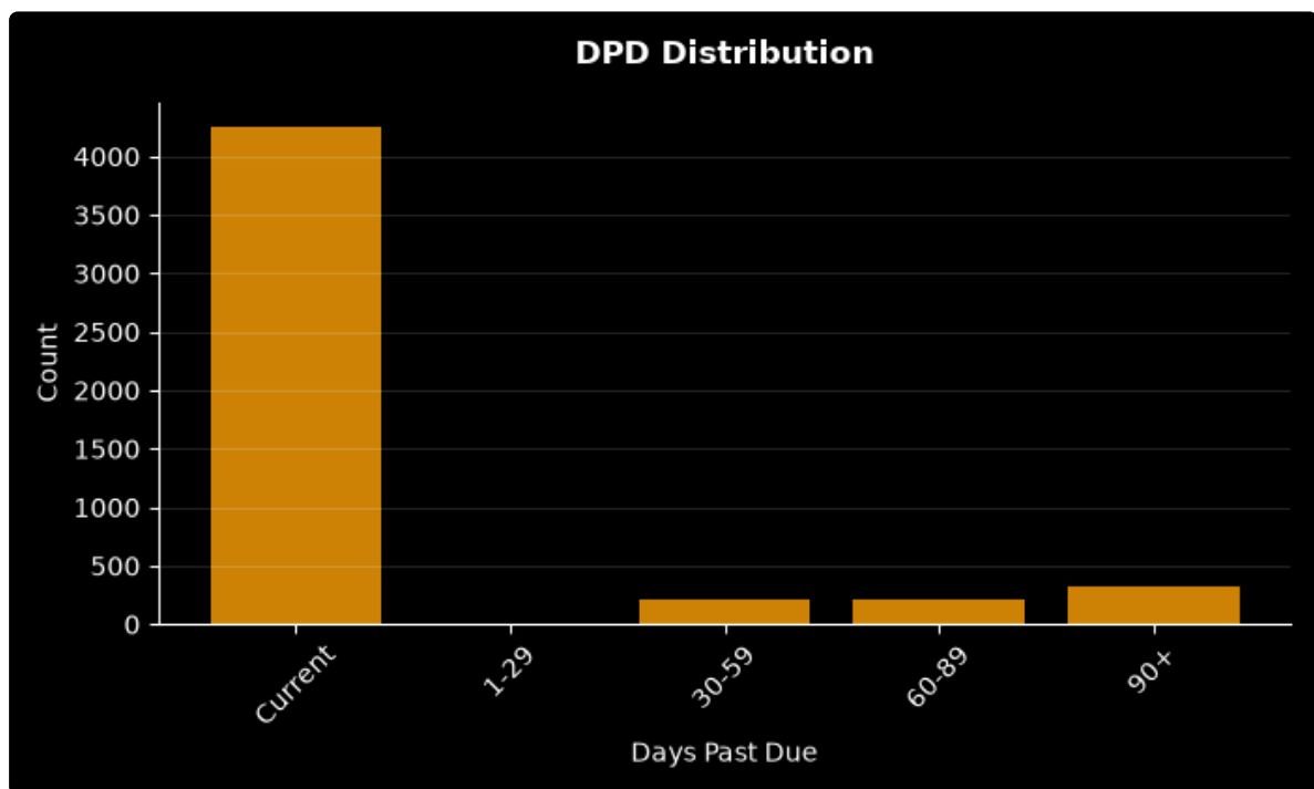
CHART_DPD_DISTRIBUTION
