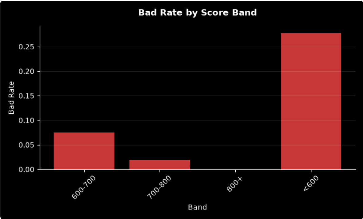
CHART_BAD_RATE_BY_SCORE_BAND
