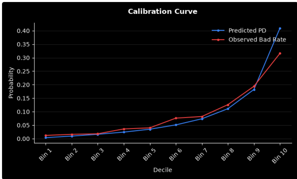
CHART_CALIBRATION
