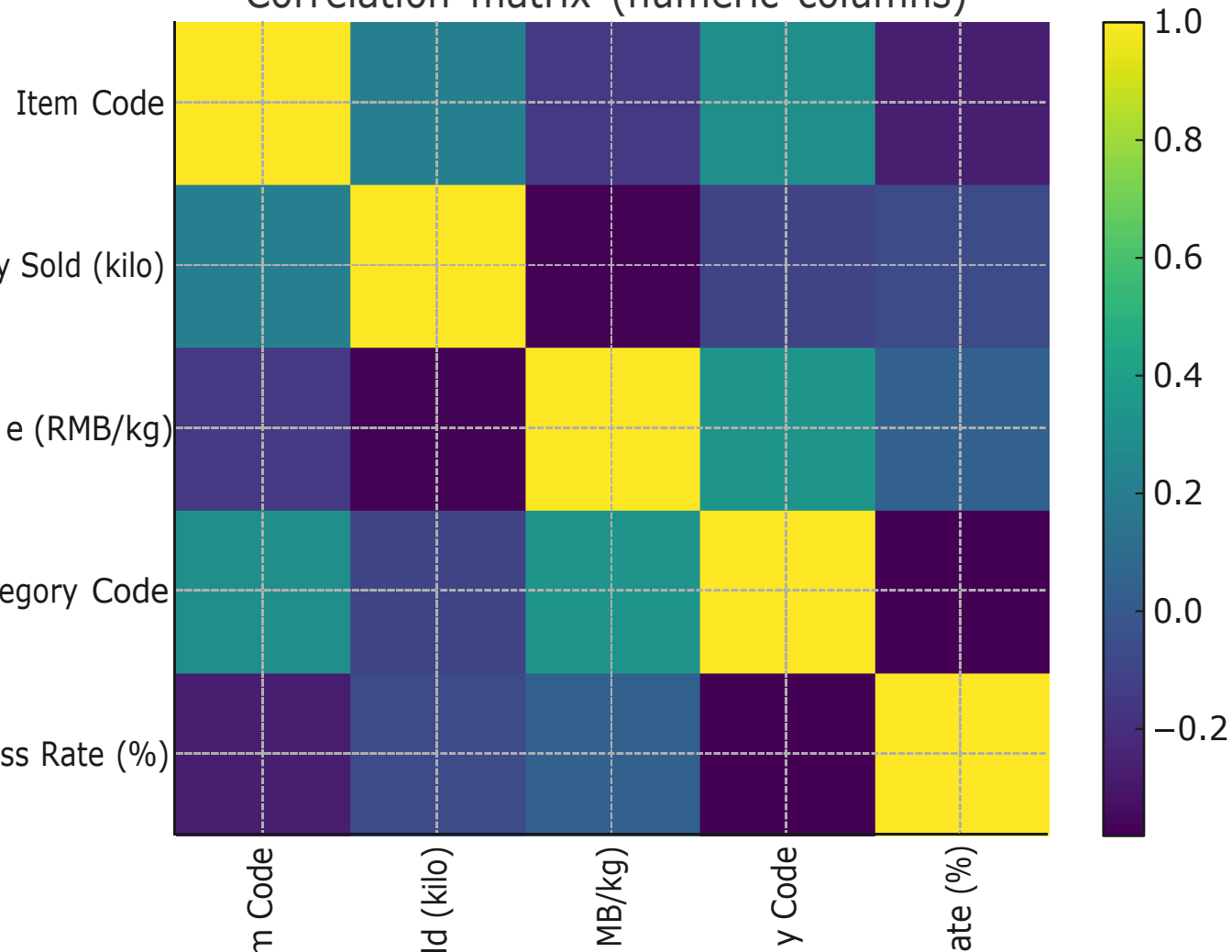
Correlation matrix (numeric columns)
