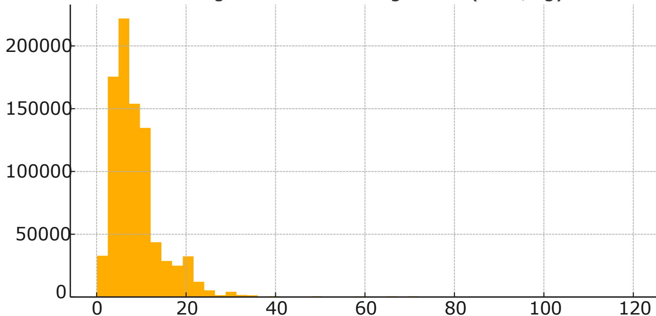
Histogram: Unit Selling Price (RMB/kg)
