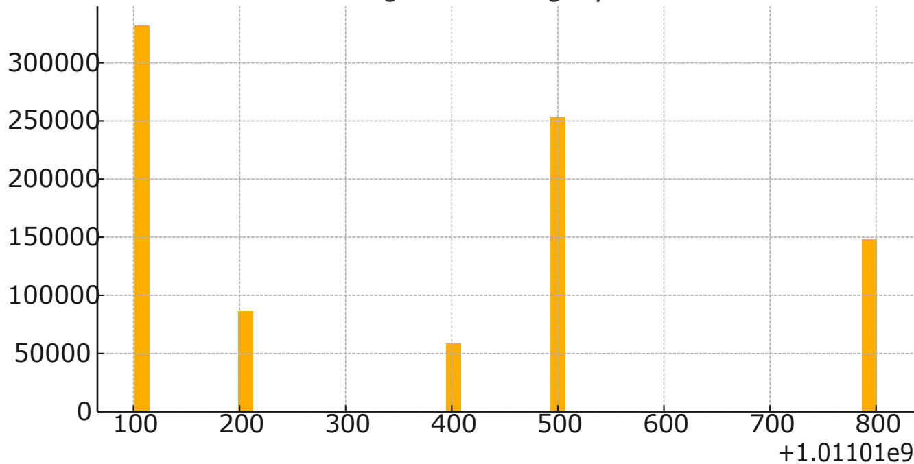
Histogram: Category Code
