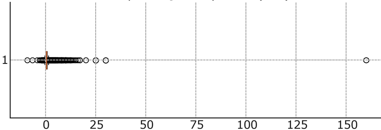
Boxplot: Quantity Sold (kilo)
