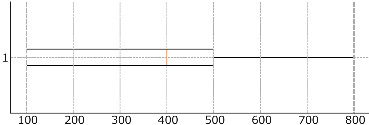
Boxplot: Category Code
