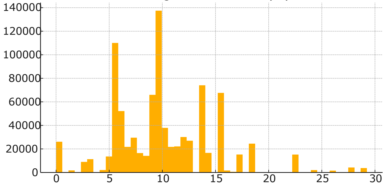
Histogram: Loss Rate (%)
