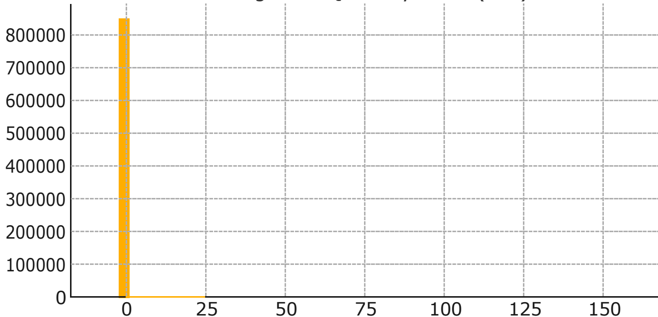
Histogram: Quantity Sold (kilo)
