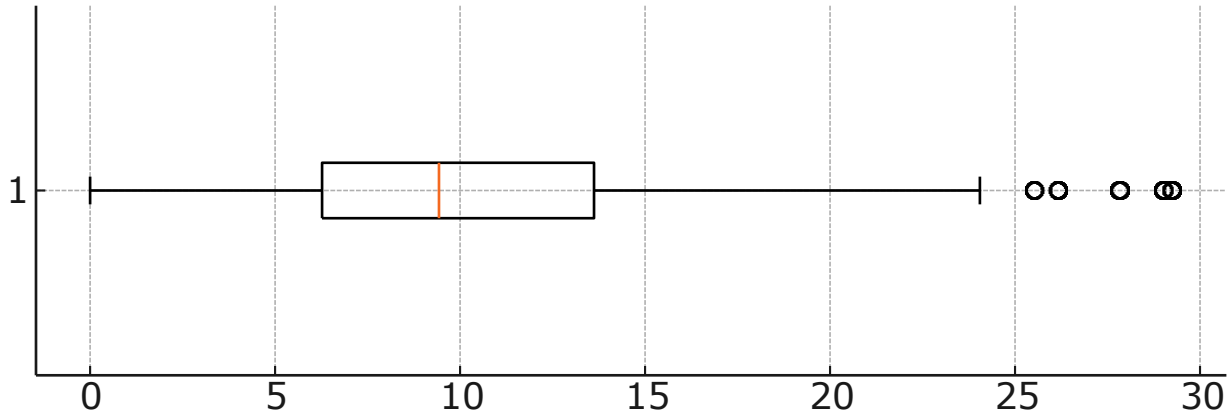
Boxplot: Loss Rate (%)
