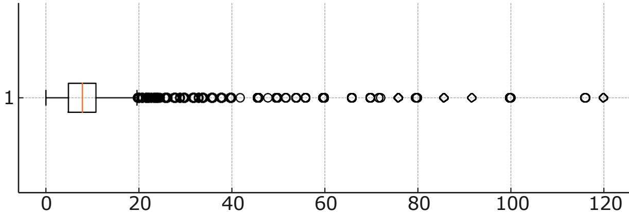
Boxplot: Unit Selling Price (RMB/kg)
