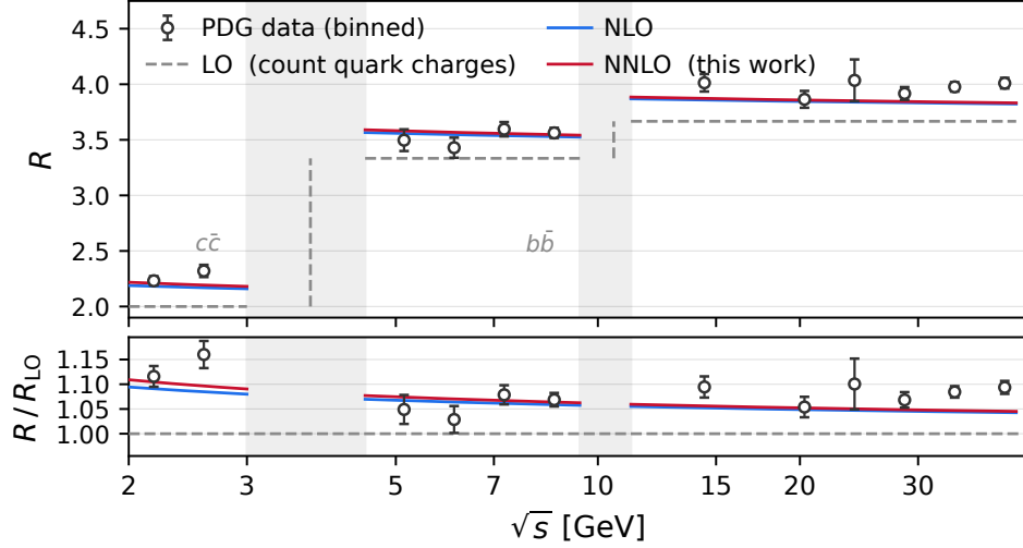
Figure 5.2: Comparison of the LO, NLO, and NNLO massless perturbative predictions for the hadronic R -ratio with the PDG data in the range 2 \lesssim \sqrt{s} \lesssim 30 GeV. The grey-shaded bands indicate the charm- and bottom-quark threshold regions. The lower panel shows the results normalised to the LO prediction, highlighting the improved overall description obtained after including the higher-order QCD corrections.
