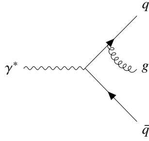
(a) Gluon emitted from the quark line.
