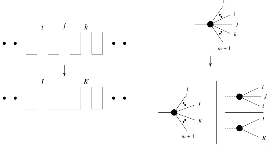
Figure 2.2: The colour connections in between parent and daughter partons before and after an emission, accompanied also by the corresponding amplitude-level factorisation, using the momenta labels.
