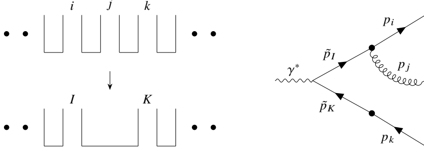
Figure 2.2: The colour connections in between parent and daughter partons before and after an emission, accompanied also by a schematic Feynman diagram using the momenta labels.
