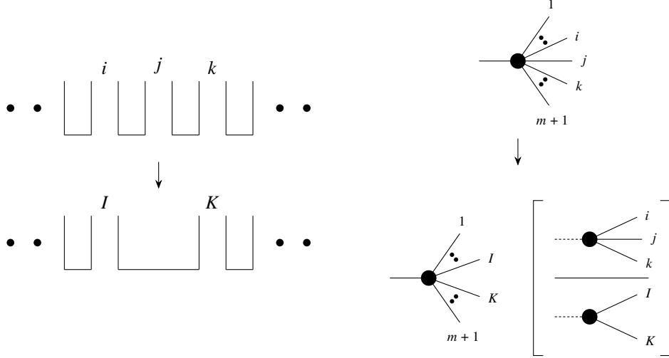
Figure 2.2: The colour connections in between parent and daughter partons before and after an emission, accompanied also by a schematic Feynman diagram using the momenta labels.
