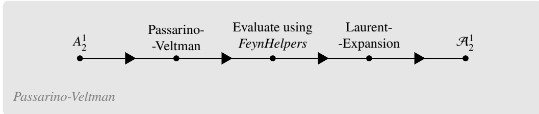
Figure 3.7: Passarino-Veltman reduction for the A_2^1 antenna integration.
