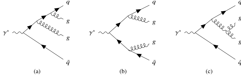
Figure 4.5: Representative tree-level Feynman diagrams for \gamma^* \rightarrow qgg\bar{q} : (a) both gluons emitted from the quark line, (b) one gluon emitted from each of the quark and antiquark lines, and (c) a diagram with the three-gluon vertex.
