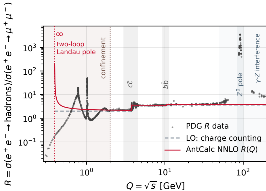
Figure 5.1: Comparison of the massless NNLO R -ratio obtained with AntCalc with the PDG data over the full energy range considered. The LO charge-counting result is shown for reference. The indicated regions highlight the low-energy non-perturbative regime, heavy-quark thresholds, and the electroweak Z^0 -pole region, illustrating the limited domain in which the massless fixed-order QCD prediction can be meaningfully compared with the data.
