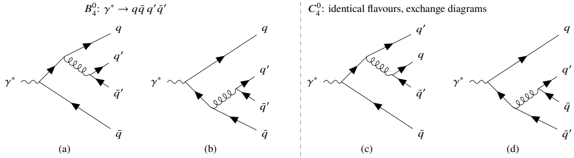
Figure 4.6: Representative tree-level Feynman diagrams for \gamma^* \rightarrow q\bar{q}q'\bar{q}' ( B_4^0 ), in which the secondary pair is produced by gluon splitting from (a) the quark line or (b) the antiquark line. For identical flavours, the exchange diagrams (c) and (d), with the final-state quarks or antiquarks interchanged, also contribute, and C_4^0 arises from their interference with the direct diagrams.
