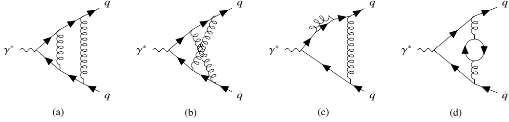
Figure 4.3: Representative two-loop Feynman diagrams for \gamma^* \rightarrow q\bar{q} : (a) planar and (b) crossed ladder, (c) a quark self-energy insertion, and (d) a closed quark loop on the gluon propagator, which gives rise to the N_f -dependent component \hat{A}_2^2 . Panel (c) is a self-energy insertion on an internal propagator, which contributes. Self-energy corrections on the external legs and tadpoles are not generated: they are scaleless for massless on-shell partons and vanish in dimensional regularisation.
