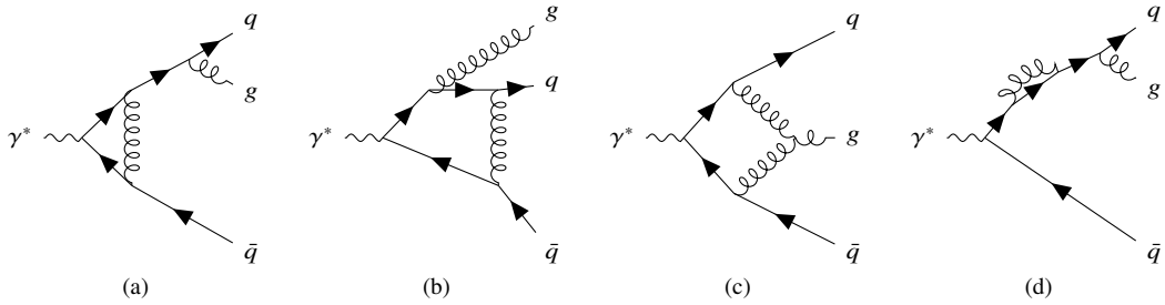
Figure 4.4: Representative one-loop Feynman diagrams for \gamma^* \rightarrow qg\bar{q} : (a) a vertex correction, (b) a box, in which the loop gluon spans the emission of the real gluon, (c) a diagram with the three-gluon vertex, and (d) a self-energy insertion on the internal quark propagator, which contributes. Self-energy corrections on the external legs and tadpoles are not generated: they are scaleless for massless on-shell partons and vanish in dimensional regularisation.
