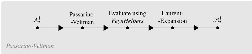
Figure 3.7: Passarino-Veltman reduction for the A_2^1 antenna integration.
