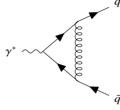
Figure 4.2: The one-loop Feynman diagram contributing to \gamma^* \rightarrow q\bar{q} (vertex correction), from which A_2^1 arises. The self-energy corrections on the external quark and antiquark legs are scaleless and vanish for massless on-shell partons in dimensional regularisation.
