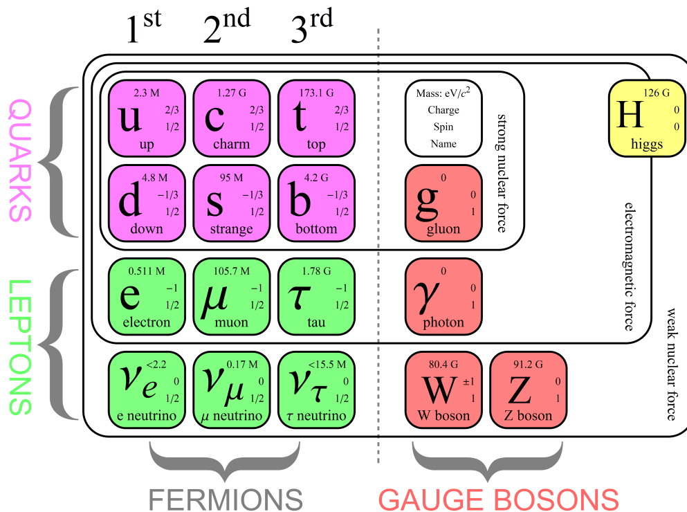
Figure 1.1: A diagram representing the Standard Model of Particle Physics. In it, the six quark flavours are visible on the top left in purple, among the fermions, and the gluon is shown in red, as the topmost of the gauge bosons. Image by Matic Lubej [1].
