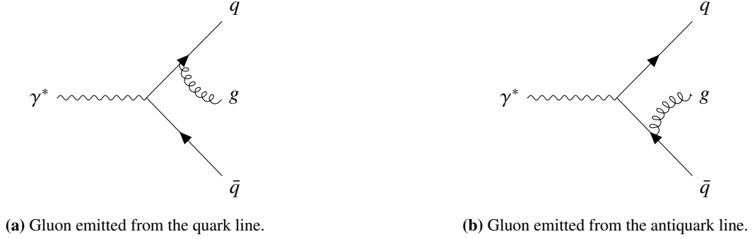
Figure 4.1: Feynman diagrams depicting the two topologies described under the A_3^0 antenna, corresponding to the process \gamma^* \rightarrow q(k_1)g(k_3)\bar{q}(k_2) .
