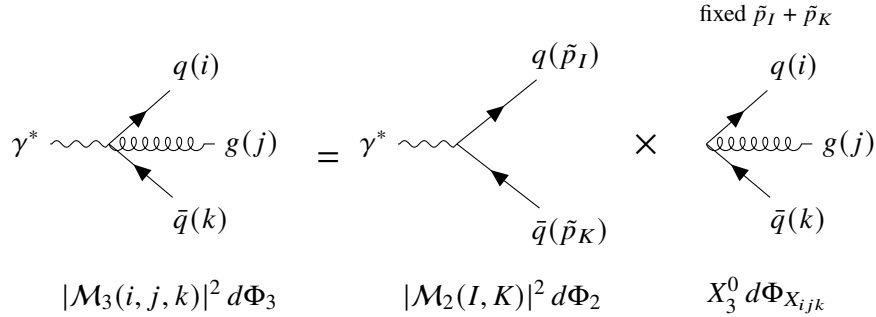
Figure 2.2: Factorisation of the squared matrix element and phase space as particle j becomes unresolved, for the NLO quark-antiquark antenna. The hard radiators i, k map onto the reduced Born momenta \tilde{p}_I, \tilde{p}_K ; the antenna function X_3^0 depends only on the antenna's own internal invariants, evaluated at fixed total momentum \tilde{p}_I + \tilde{p}_K .
