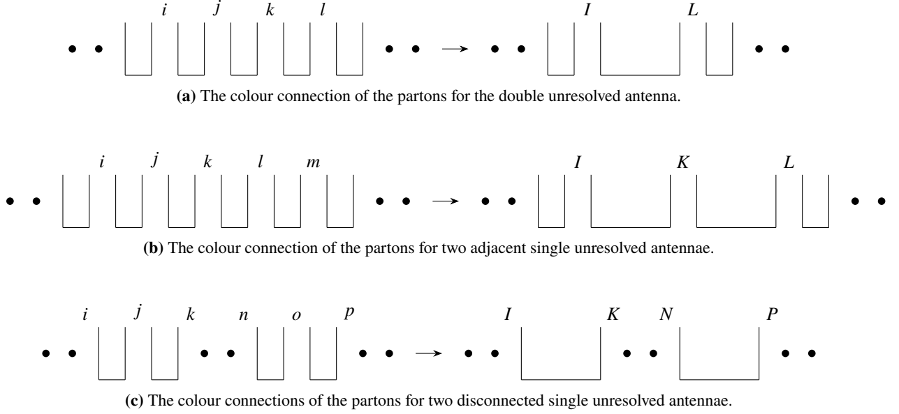
Figure 2.3: The three characteristic double-unresolved colour-connection configurations at NNLO: (a) two colour-connected unresolved partons, (b) two adjacent single-unresolved antennae, and (c) two disconnected single-unresolved antennae.
