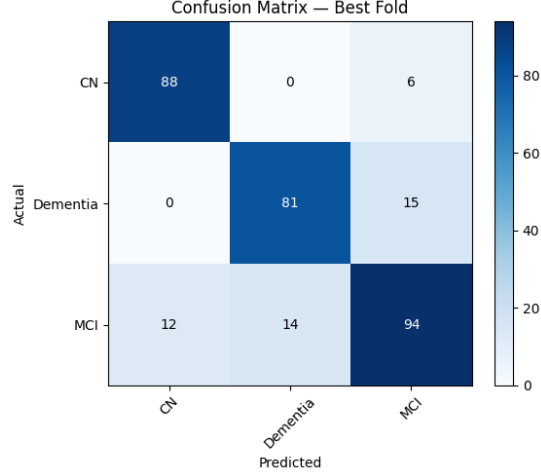
Fig. 28: Fold 4 confusion matrix, GPU-trained model.
