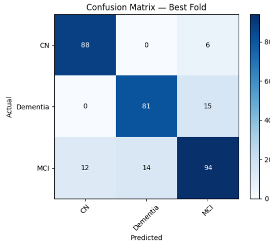
Fig. 28: Fold 4 confusion matrix, GPU-trained model.
