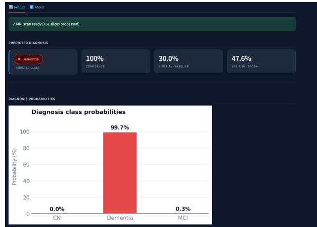
Fig. 36: Deployed dashboard, prediction output for the held-out verification patient.
