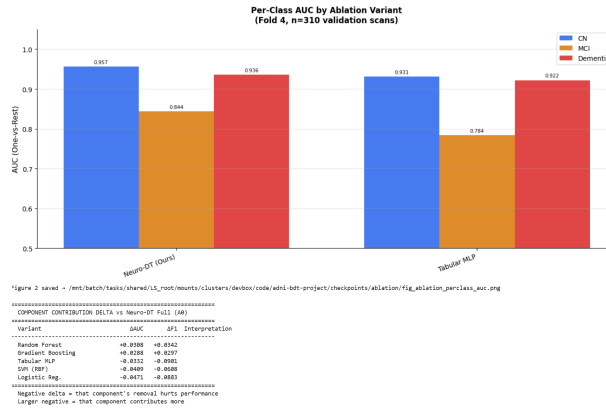
Fig. 14: CPU-feasible ablation results, per-class AUC.
