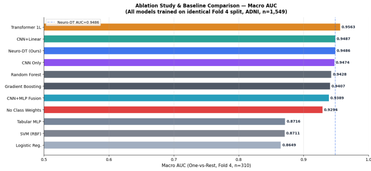
Fig. 26: Ablation study, AUC comparison across all 11 variants.
