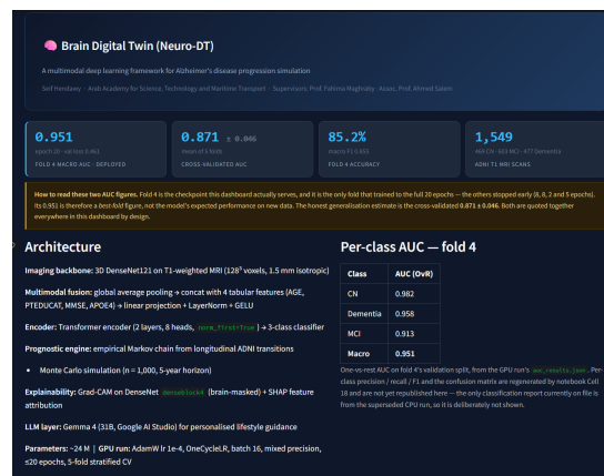
Fig. 37: Deployed dashboard, “About” / model-info panel.
