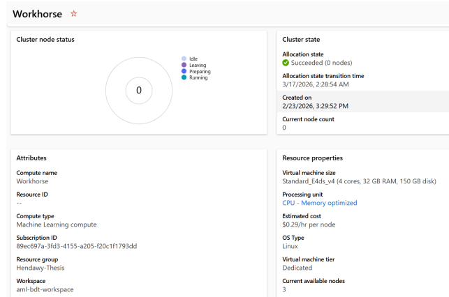
Fig. 10: Azure Machine Learning Workhorse compute cluster specification.
