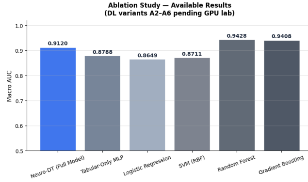
Fig. 16: CPU-feasible ablation results, bar chart.
