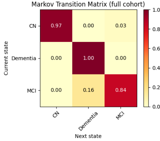
Fig. 19: Markov transition matrix heatmap, full cohort, CPU run.
