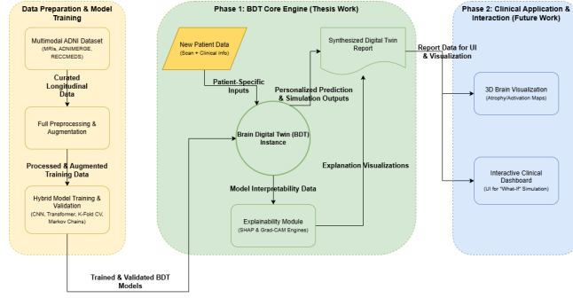
Fig. 1: Neuro-DT framework as originally proposed.
