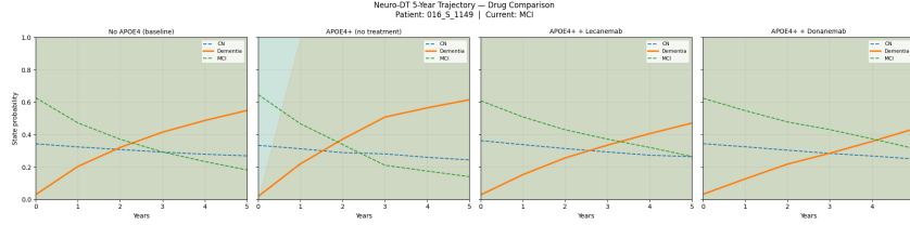
Fig. 20: What-if simulation trajectories for Patient 016_S_1149 under the CPU-trained model.
