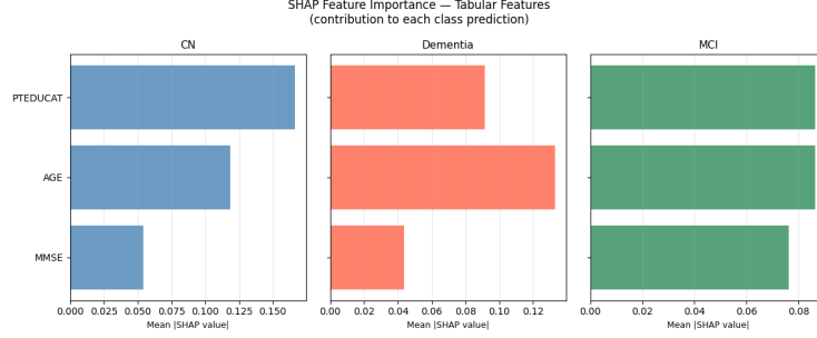
Fig. 17: SHAP tabular feature attribution (CPU-trained model).
