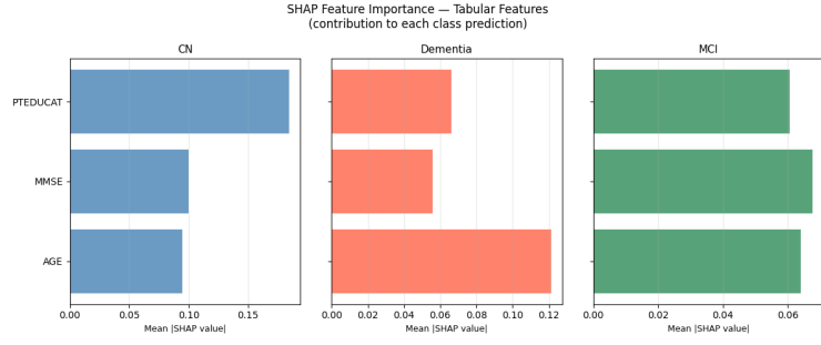
Fig. 29: SHAP tabular feature attribution, GPU-trained model.
