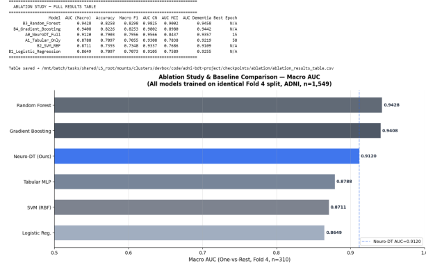
Fig. 13: CPU-feasible ablation results, horizontal comparison chart.
