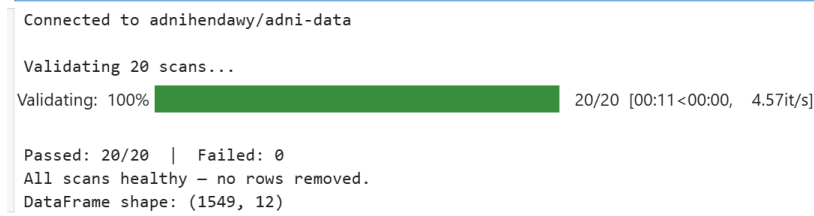
Fig. 6: DICOM integrity validation log (pipeline stage 3).
