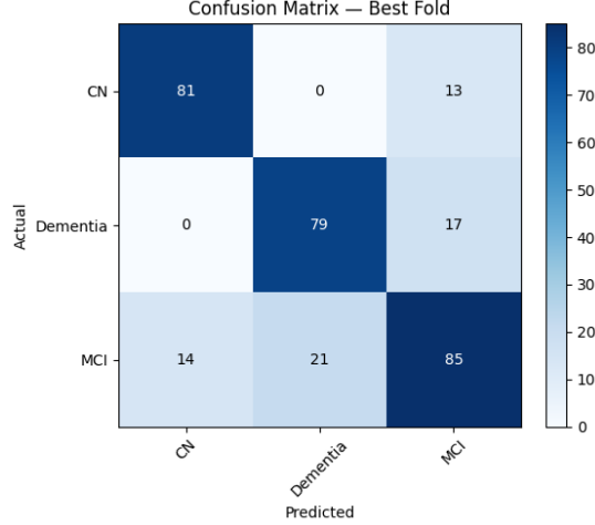
Fig. 12: Fold 4 confusion matrix (CPU-trained model).
