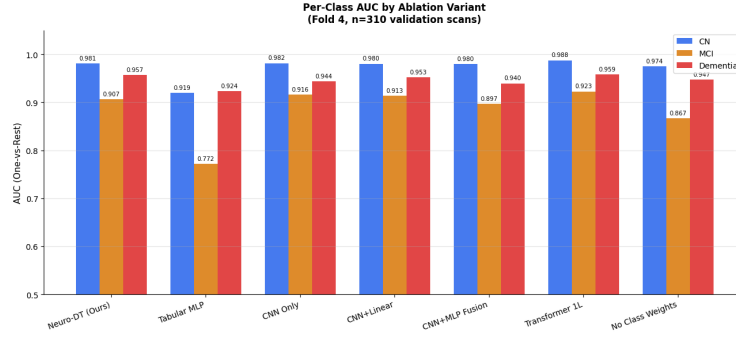
Fig. 27: Ablation study, per-class AUC grouped chart.
