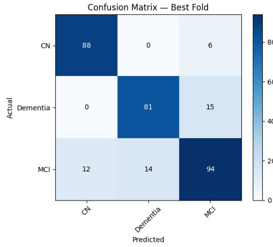
Fig. 28: Fold 4 confusion matrix, GPU-trained model.
