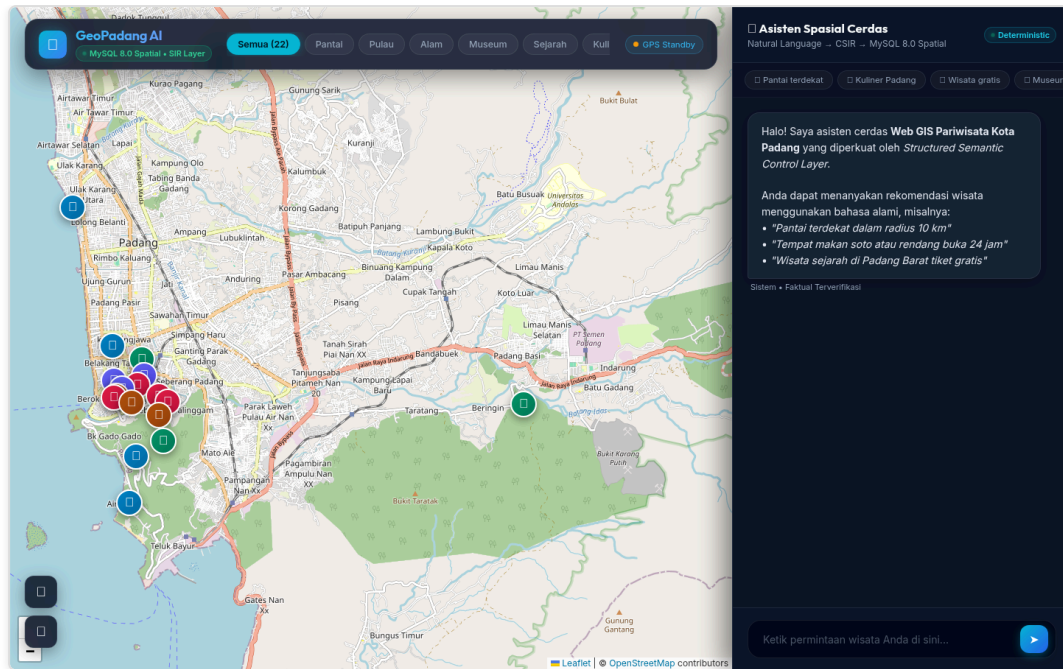
Figure 2. Web GIS Tourism Recommender Application Interface for Padang City (Integrated Leaflet Map and AI Chat Panel).
