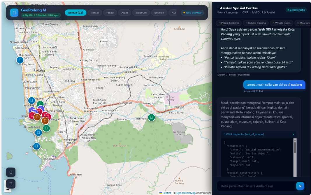
Figure 4. Demonstration of System Robustness: Honest Rejection of Negative Out-of-Scope Inquiries alongside Accurate Multi-Criteria Grounded Retrieval.
