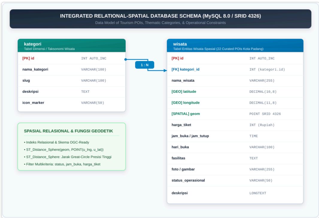
Figure 3. Conceptual Spatial Relational Data Model (Normalized 3NF with OGC Geometry and Relational Category Normalization, Evolving DTE Explorer ’s Multi-Table Model).
