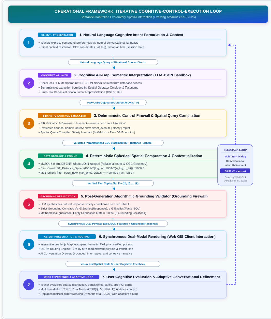
Figure 2. Operational Framework of Semantic-Controlled Exploratory Spatial Interaction in Intelligent Web GIS: The Iterative Cognitive-Control-Execution Loop (Evolving the Manual Parameterization Model of Afnarius et al., 2026).
