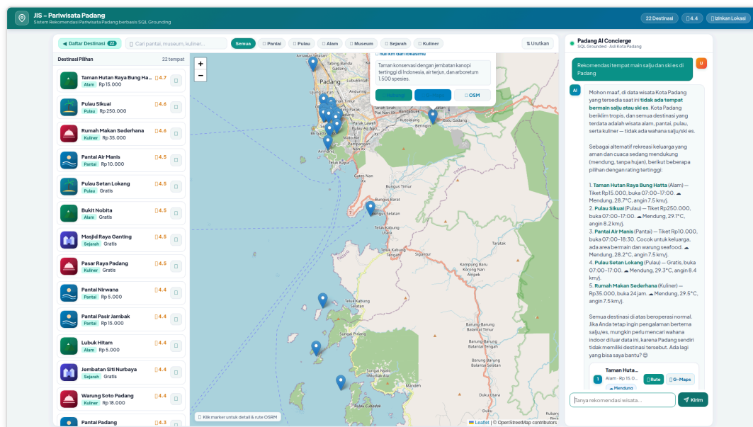
Figure 4. Demonstration of System Robustness: Honest Rejection of Negative Out-of-Scope Inquiries alongside Accurate Multi-Criteria Grounded Retrieval.
