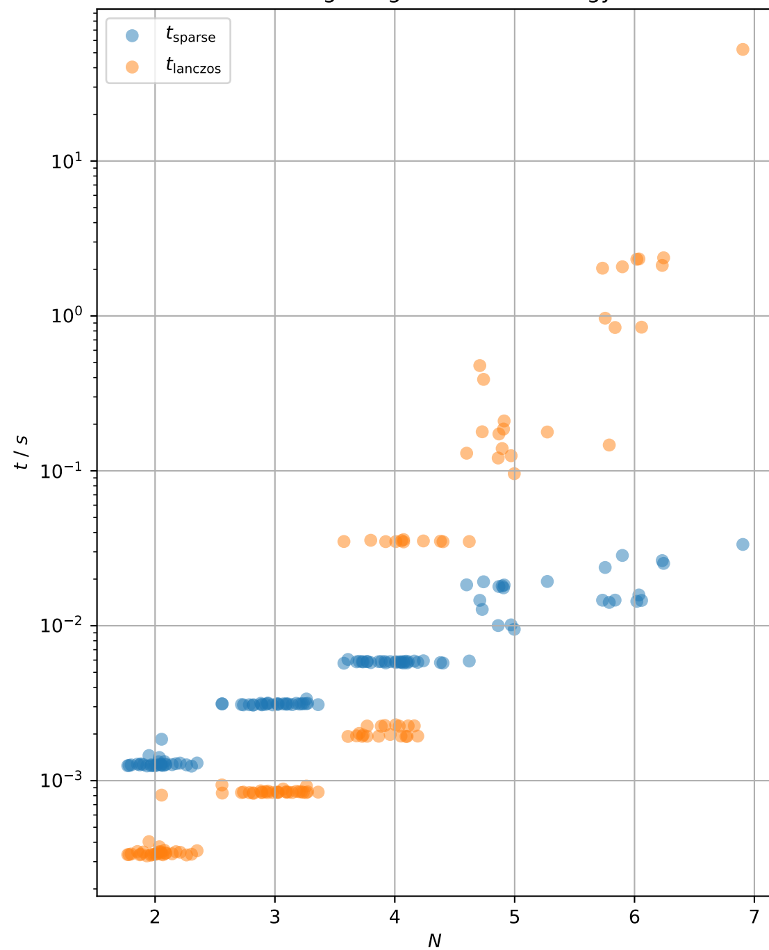
Finding the ground state energy
