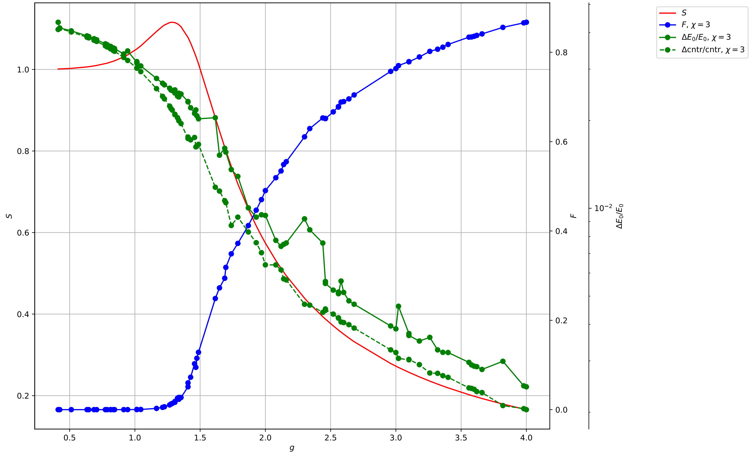
Entanglement entropy, Fidelity, rel.err. E_0
