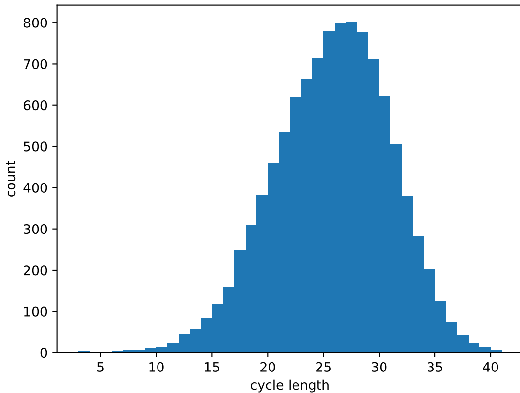
Graph with 61 nodes.
