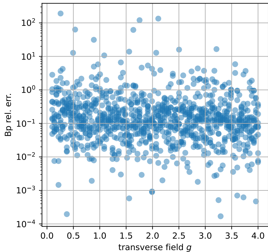
BP on \langle \psi | (\text{TFI}_+ + \text{TFI}_-) | \psi \rangle for varying transverse field g . hex(2,1)-graph. Random state |\psi\rangle .
