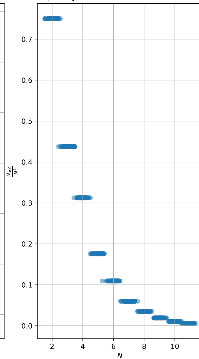
Sparsity: Saved values to matrix size
