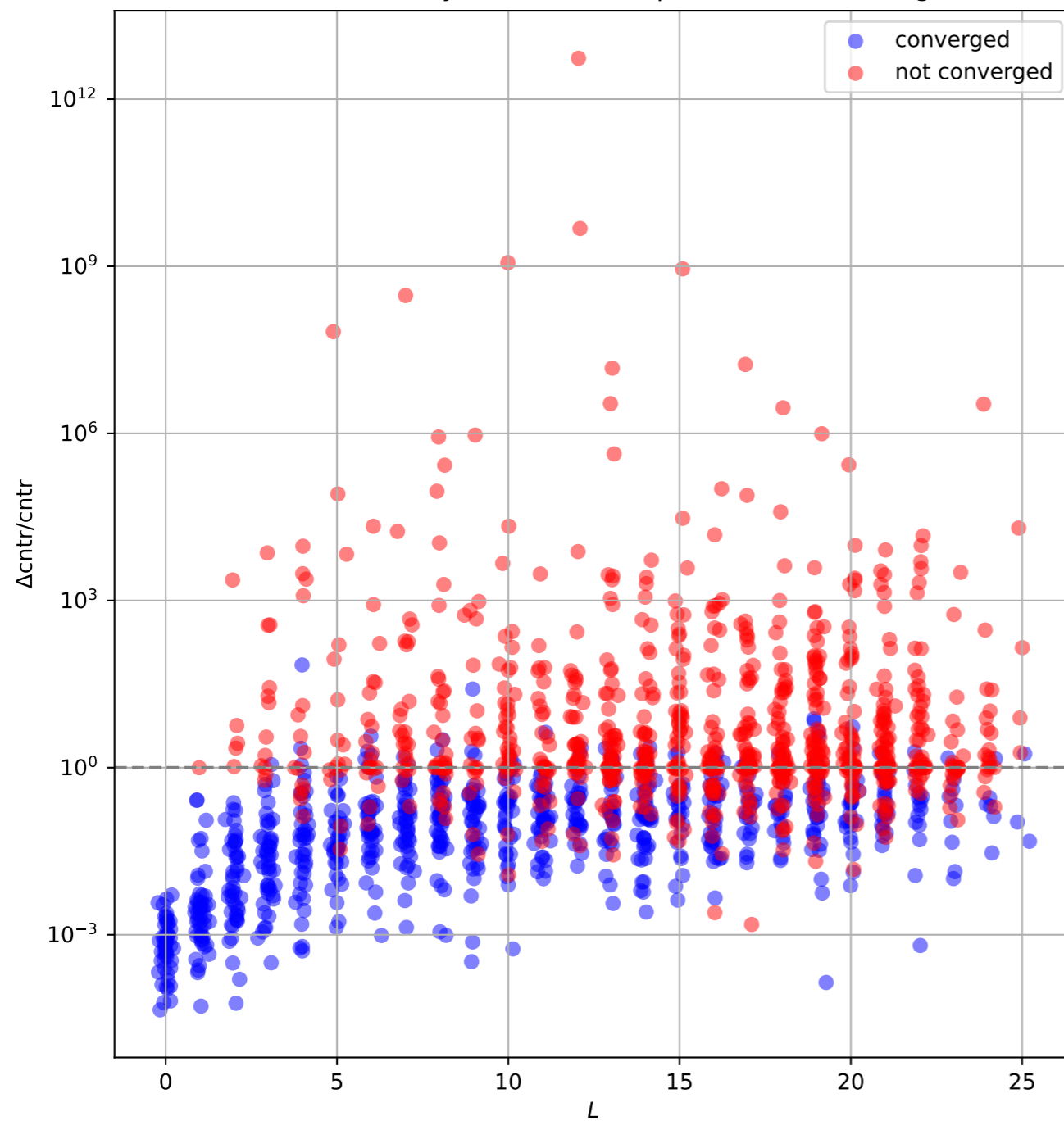
rel.err.BP on heavyhex(2,2) with operator chain of length L
