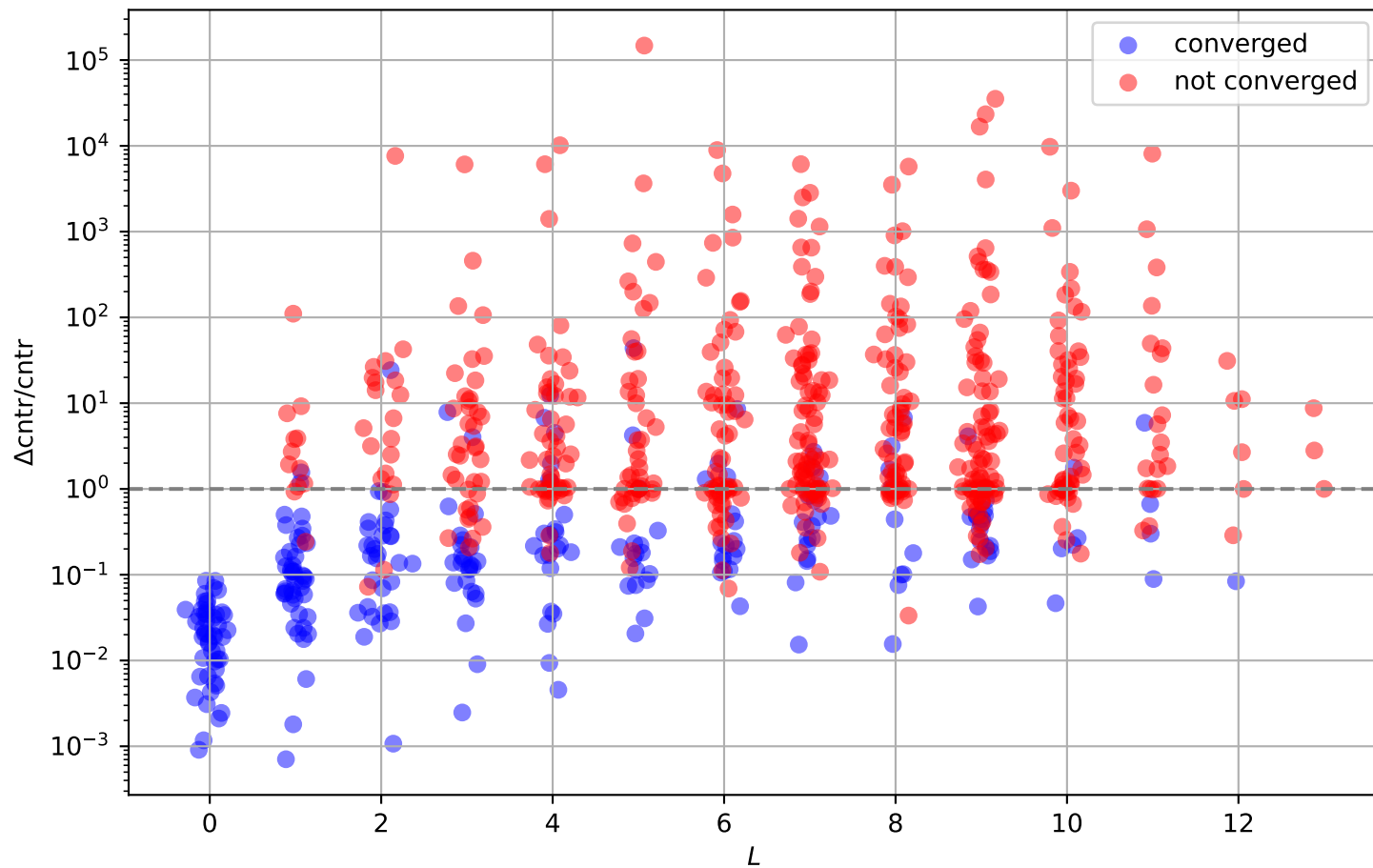
rel.err.BP on hex(2,2) with operator chain of length L
