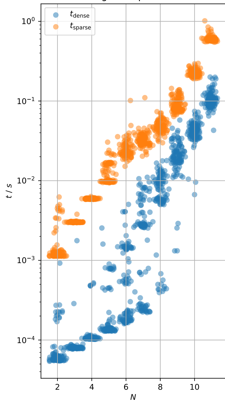
Forming the representation
