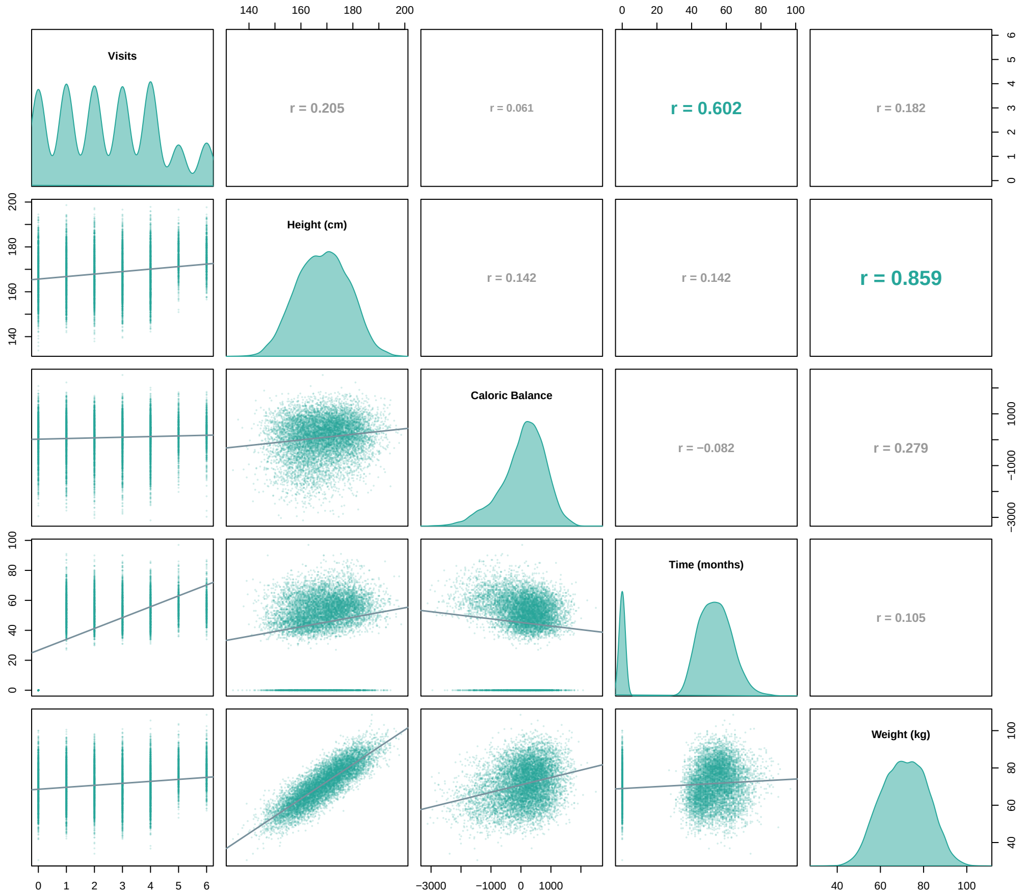
Pairwise Scatter Matrix with Correlations
