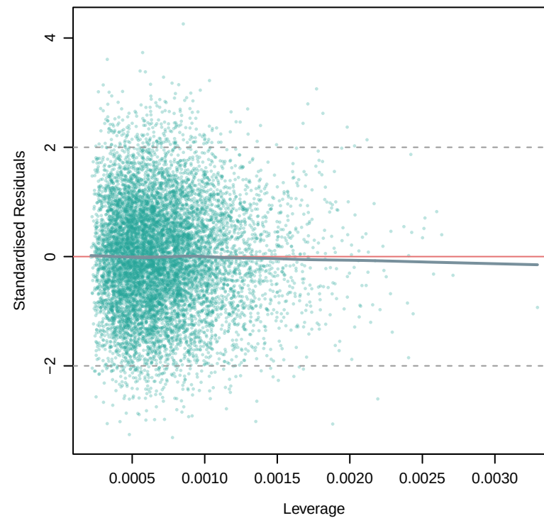
Residuals vs Leverage
