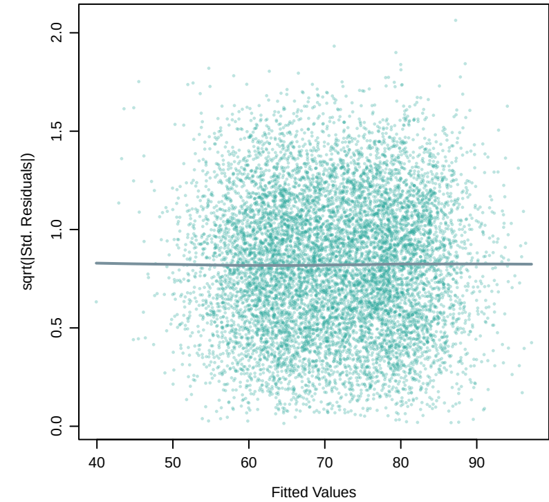
Scale-Location
