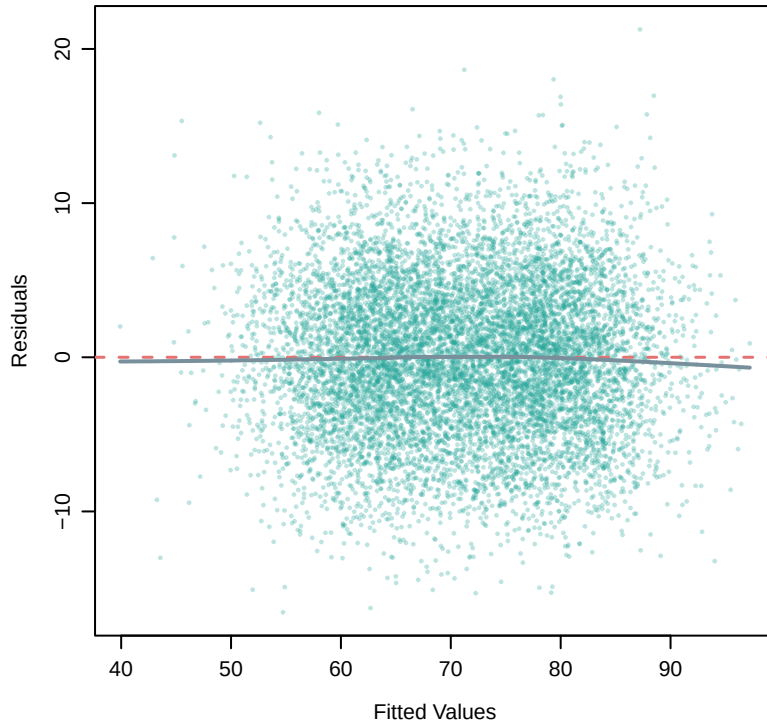
Residuals vs Fitted
