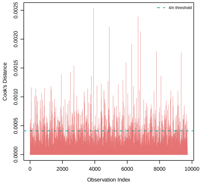
Cook's Distance
