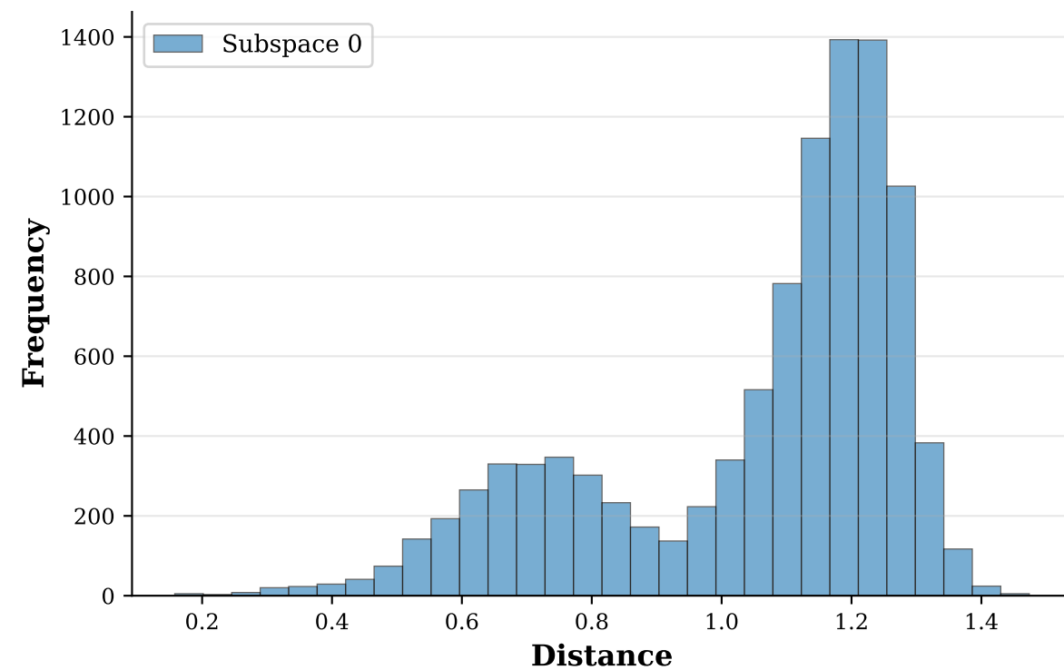
Distribution of Distances per Subspace (nbits=10) DEEP
