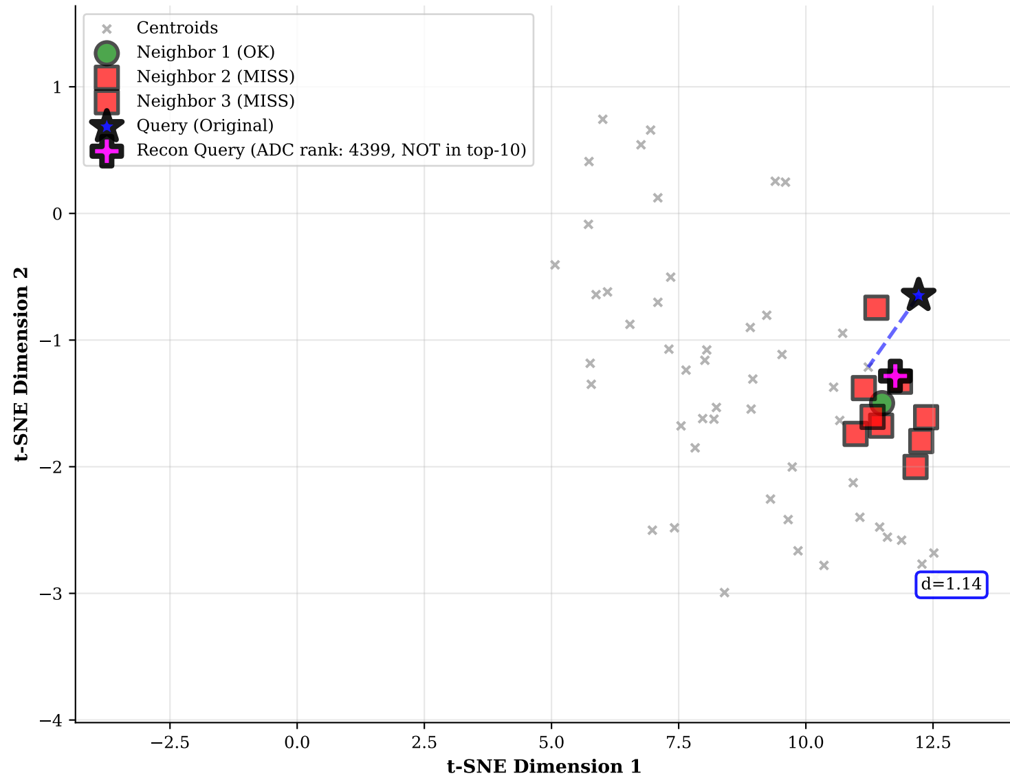
Reconstructed Vectors (nbits=8)
