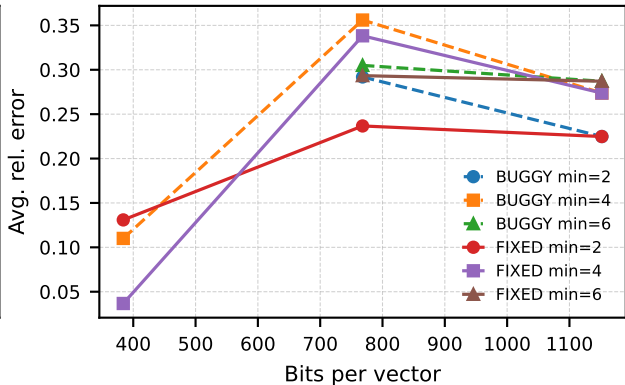
Deep1B — max_bits=16
