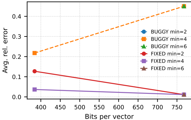
Deep1B — max_bits=8
