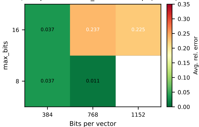
VAQ Deep1B — min rel_error heatmap [FIXED]
