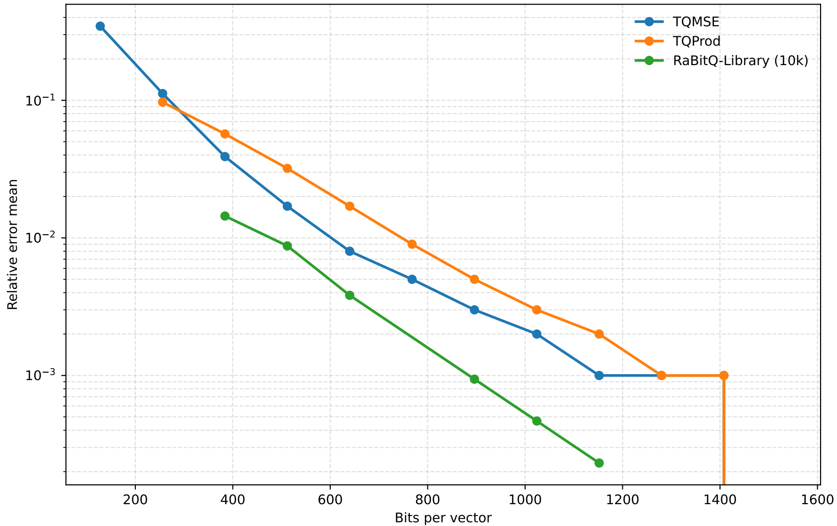
BigANN relative error: TurboQuant vs RaBitQ-Library
