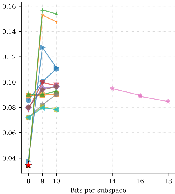
Std dev of relative error
