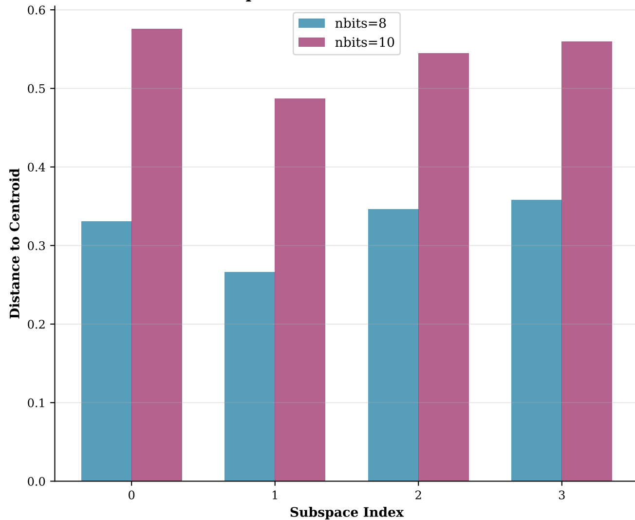
Subspace Distances to Centroids
