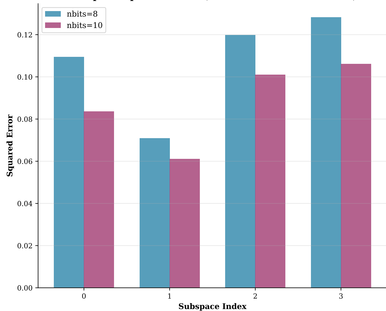
Subspace Squared Errors (What Matters for Full Error)
