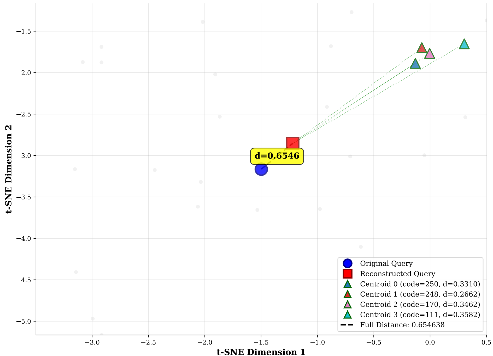
t-SNE: Original vs Reconstructed Query with Centroids DEEP Dataset, Query 2 (nbits=8, n_subquantizers=4)
