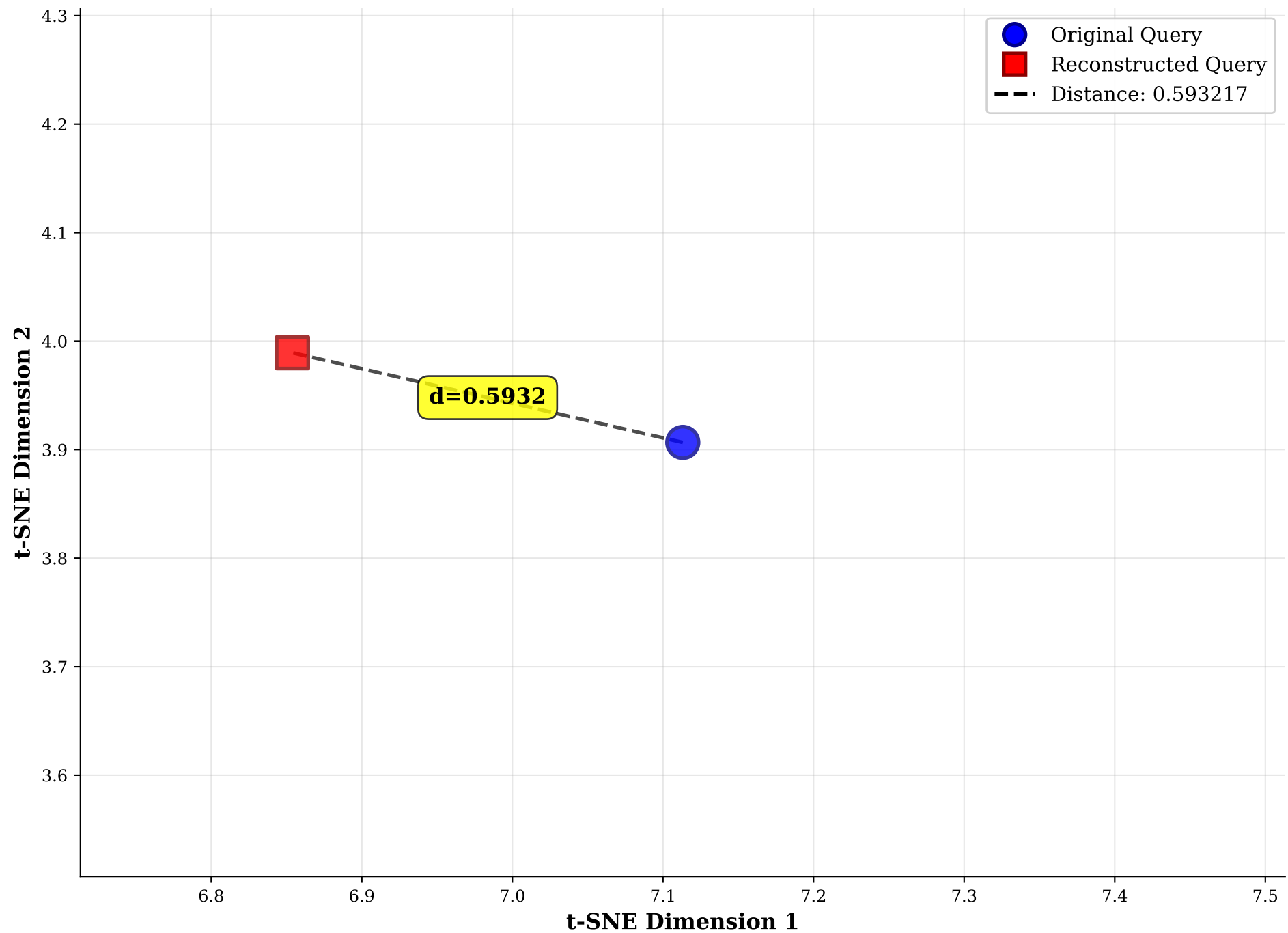
t-SNE: Original vs Reconstructed Query DEEP Dataset, Query 2 (nbits=10, n_subquantizers=4)
