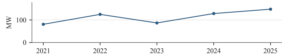
邳州35 kV
