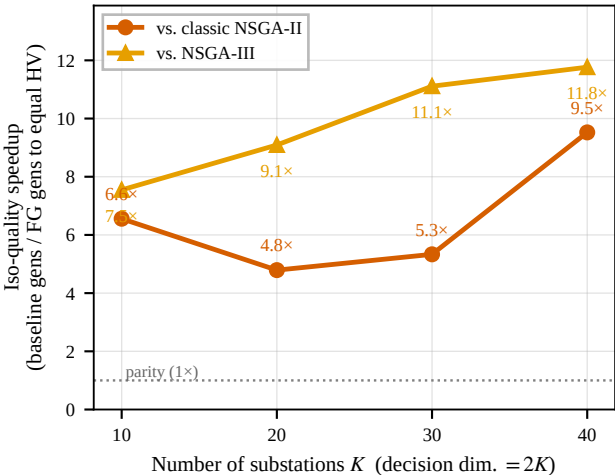
Convergence speedup vs. scale
