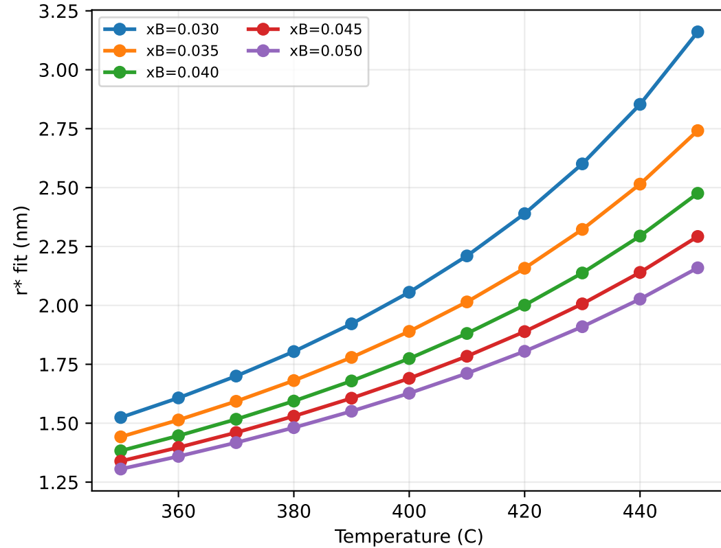
Fitted critical-radius trend
