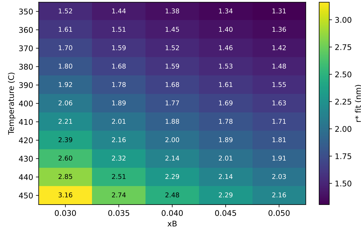
Fitted critical-radius trend
