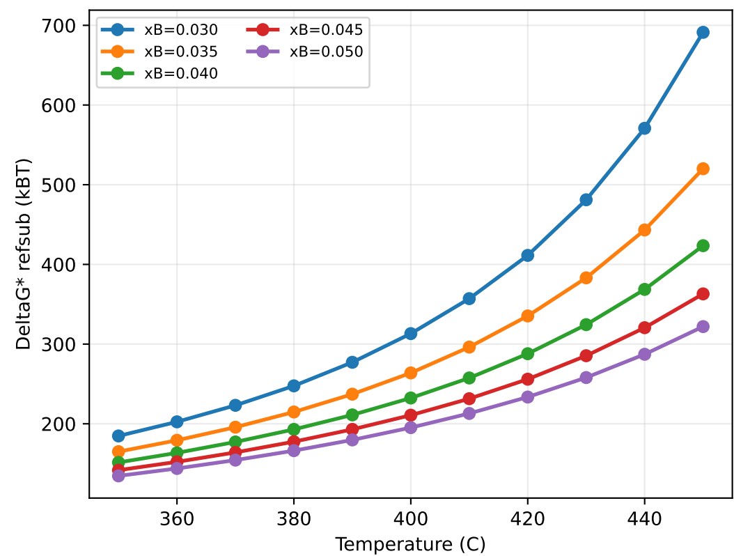
CNT barrier trend
