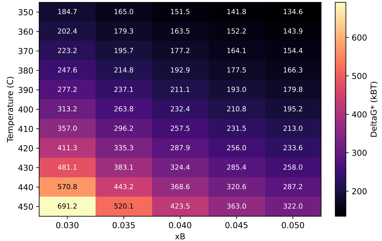
CNT barrier trend
