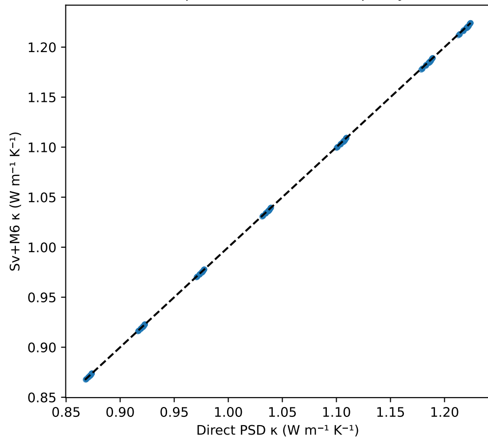
Compressed vs direct PSD parity
