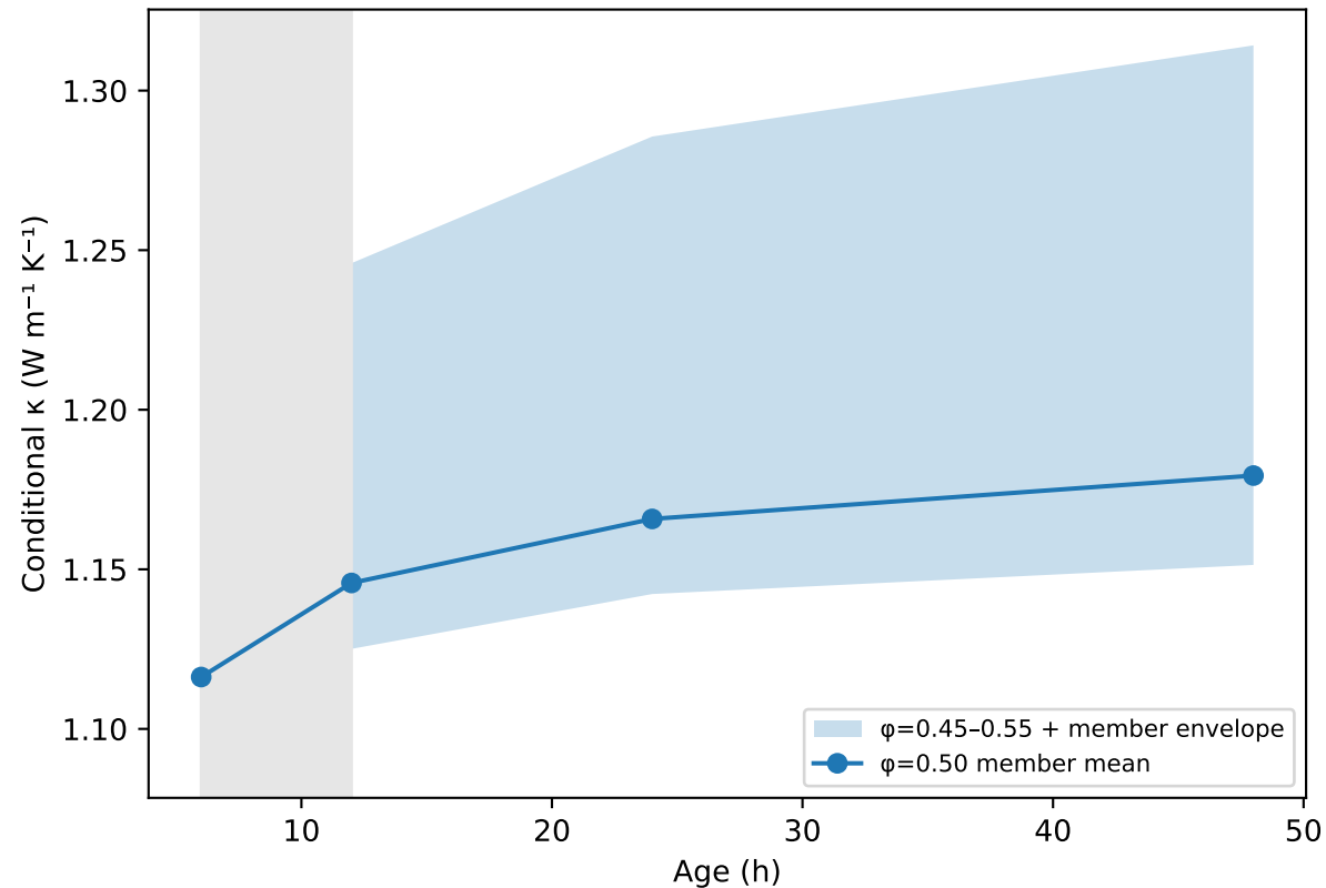
No-refit true-area sensitivity envelope, 303.15 K
